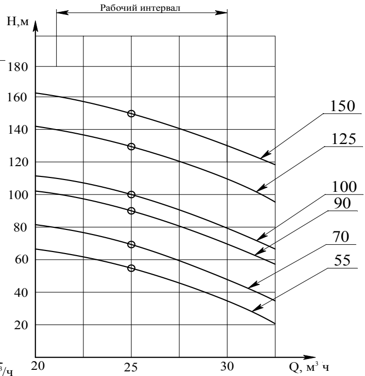
2ЭЦВ 8-40 и ЭЦВ 8-40
